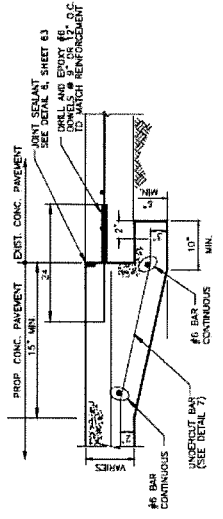
8 SECTION - TYP. PAVEMENT TIE-IN NOT TO SCALE
