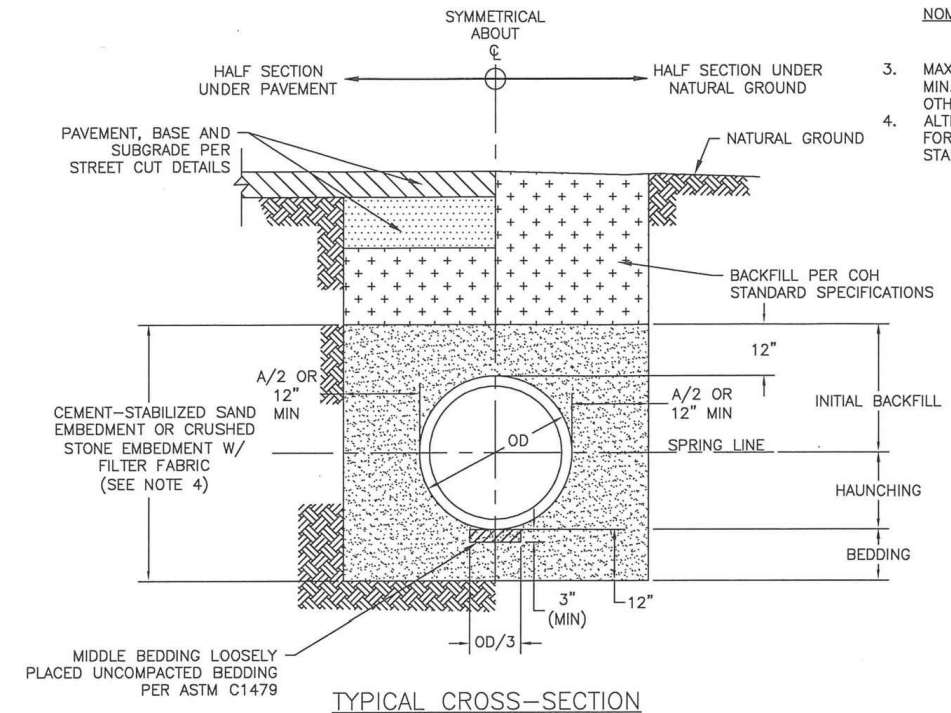
TYPICAL CROSS-SECTION
